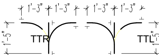
LIFT AND TURN SWITCHES MAX CAP 1500 LBS.
