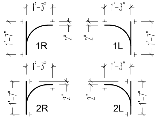
1500 LB. CAPACITY AUTO & GEAR SWITCHES
